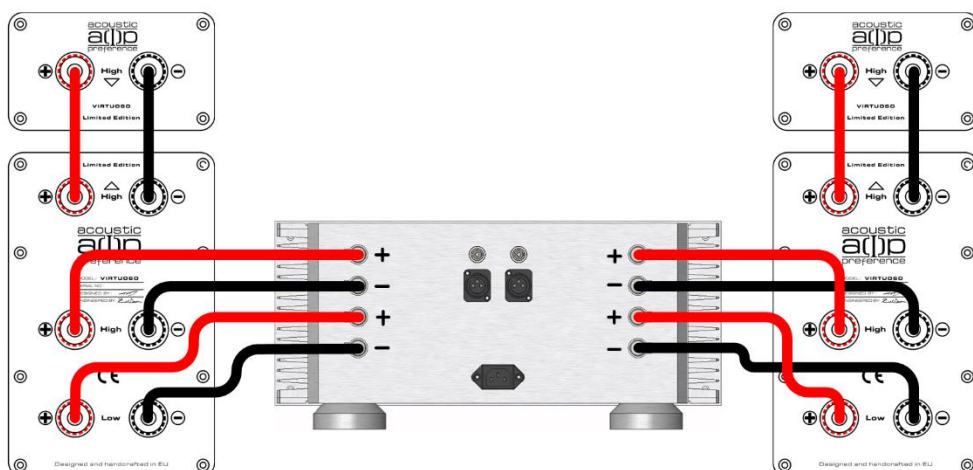
Figure 2: Bi-wire connection with single stereo amplifier. Remove jumpers-bridges.
