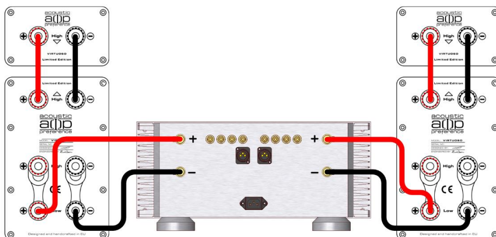
Figure 1: Connection with single stereo amplifier. Use jumpers/bridges.
